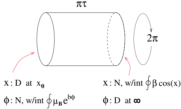
Figure 14. The annulus worldsheet describing a macroscopic loop probing a D-particle
