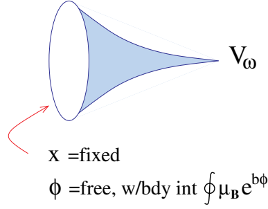
Figure 11. The disk one-point function of a tachyon perturbation is the leading-order contribution to the process whereby an incoming tachyon is absorbed by a macroscopic loop operator.
