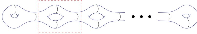
Figure 1. Each handle, except the end ones, contributes three closed string propagator tubes to the surface. Each tube has a length and a helical twist angle. The two end handles together contribute only three tubes, and so the number of moduli is 6h - 6 .
