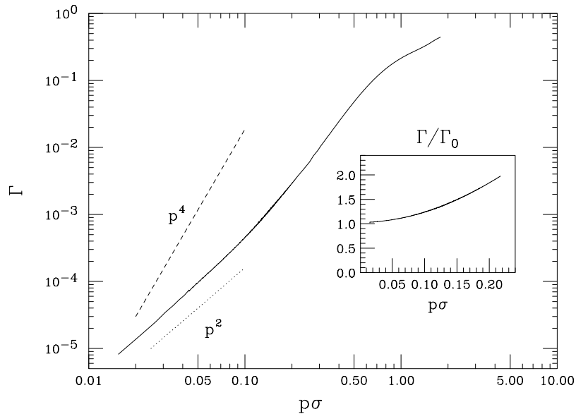
Figure 6. Peak width vs. p , for \rho = 0.6\sigma^{-3} . The inset shows that \Gamma_0(p) is the dominant contribution at small p .
