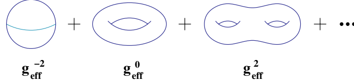
Figure 2. The string loop expansion. go
