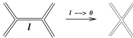
Figure 6. Collapse of a line takes us to a boundary of moduli space.
