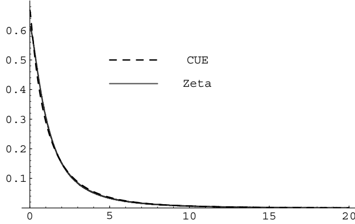
Figure 3. The CUE value distribution of |Z| corresponding to N = 12 (that is, U(12) ) (dashed), with numerical data for the value distribution of |\zeta(1/2 + it)| (solid) near t = 10^6 .
