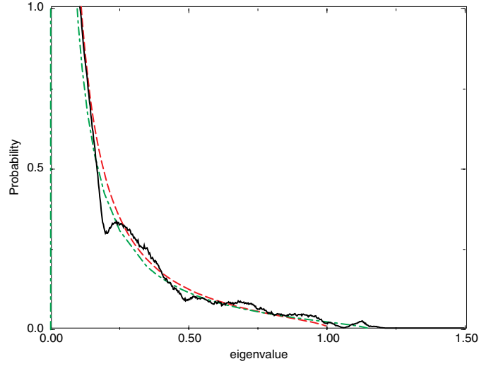
Figure 1. Density of eigenvalues of a Euclidean Random Matrix in three dimensions, density \rho = 1 . The function f is f(x) = (2\pi)^{-3/2} \exp(-x^2/2) , and the matrix is defined from eq.(48). The full line is the result of a numerical simulation with N = 800 points, averaged over 100 samples. The dashed line is the result from the high density expansion. The dash-dotted line is the result from the Gaussian variational approximation (RPA) to the field theory.
