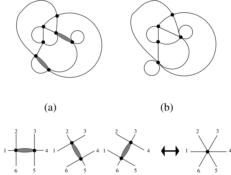
Figure 4. A 4-valent planar graph with hard dimers, represented by thickened edges. The corresponding graph obtained by shrinking the dimers (b) has both 4-valent and 6-valent vertices. The correspondence is three-to-one per dimer, as shown.
