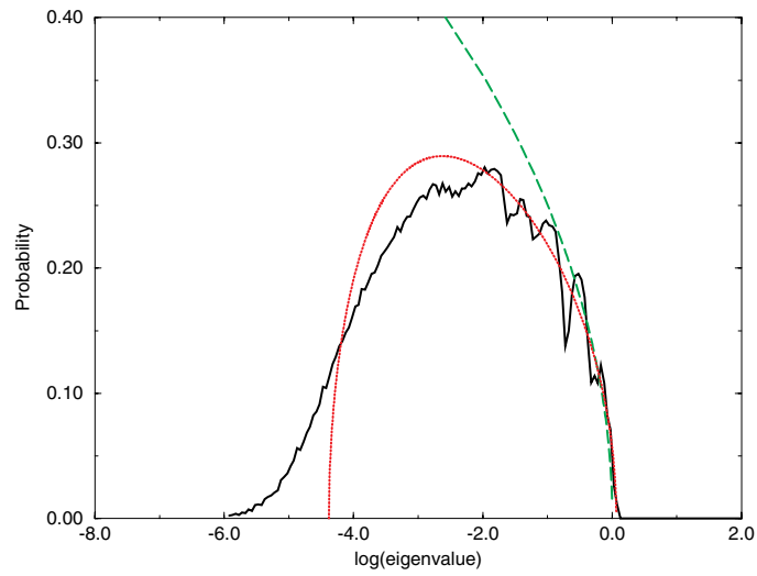
Figure 2. Density of the logarithm (in base 10) of the eigenvalues of a Euclidean Random Matrix in three dimensions, density \rho = 1 (same data of the previous figure). The dashed line is the result from the high density expansion. The dotted line is the result from the Gaussian variational approximation (RPA) to the field theory.
