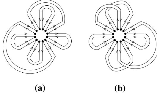
Figure 2. An example of planar (petal) diagram (a) and a non-planar one (b). Both diagrams have n = 2p = 12 half-edges, connected with p = 6 edges. The diagram (a) has p + 1 = 7 faces bordered by oriented loops, whereas (b) only has 3 of them. The Euler characteristic reads 2 - 2h = F - E + 1 ( V = 1 in both cases), and gives the genus h = 0 for (a), and h = 2 for (b).
