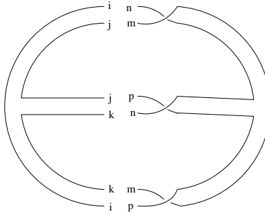
Figure 6. Contracting two cubic vertices in the double line notation: the N contribution.
