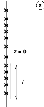
Figure 1. A typical Dirac spectrum. To derive the Banks-Casher relation we integrate the resolvent over the rectangular contour in this figure. (Figure taken from [45].)
