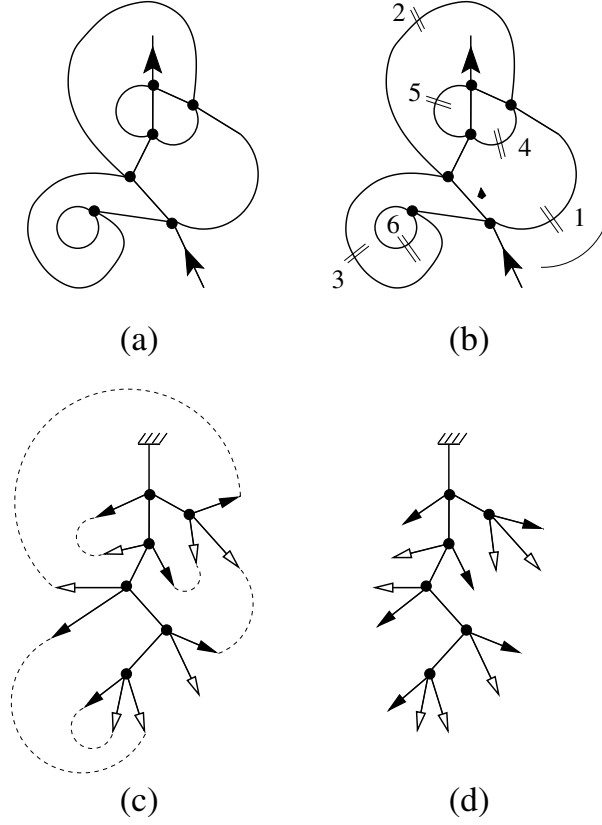
Figure 6. Illustration of the bijection between two-leg planar 4-valent graphs and rooted blossom trees. Starting from a two-leg graph (a), we apply the iterative cutting procedure, which here requires turning twice around the graph. In (b), the indices indicate the order in which the edges are cut during the 1st turn (1, 2, 3) and 2nd turn (4, 5, 6). Each cut edge is replaced by a black/white leaf pair (c), while the in-coming leg is replaced by a leaf and the out-coming one by a root, finally leading to a blossom tree (d). Conversely, the matching of black and white leaves of the blossom tree (d) rebuilds the edges of (a).
