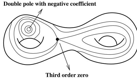
Figure 5. Riemann surface with the flow pattern of a horocyclic quadratic differential.
