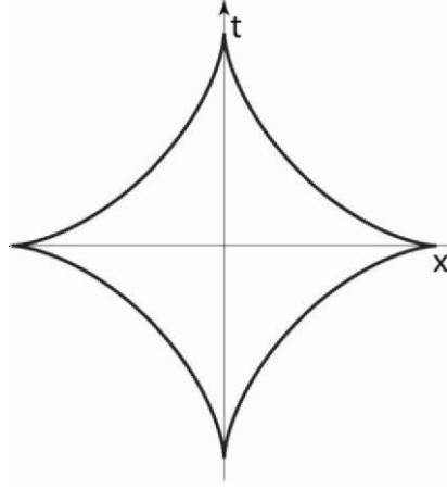
Figure 2. The region of the x - t plane in which \rho(x, t) = 0 for the EFP instanton for free fermions is shown. The boundary of the region is given by an astroid x^{2/3} + (\pi\rho_0 t)^{2/3} = R^{2/3} .
