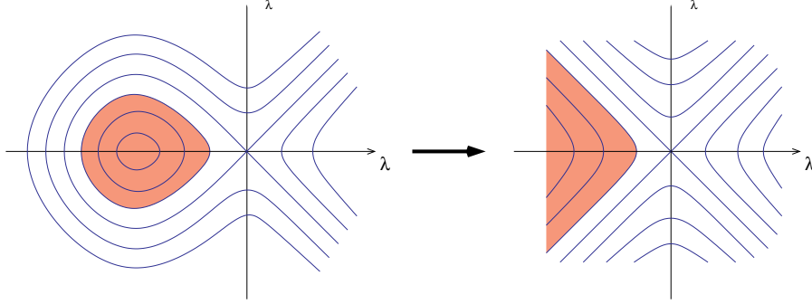
Figure 9. Phase space portrait of the classical limit of the free fermion ground state. The contours are orbits of fixed energy; the shaded region depicts the filled Fermi sea.
