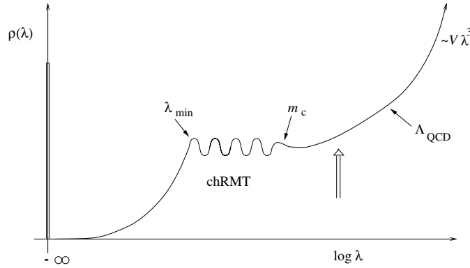
Figure 2. Schematic picture of the average spectral density of QCD Dirac operator. (Taken from [46].)
