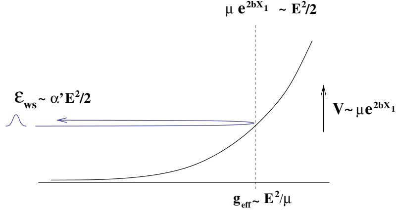
Figure 4. Scattering of a tachyon excitation off the tachyon background.
