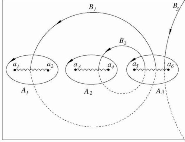
Figure 1. The A and B cycles for a genus 2 spectral curve ( p = 3 ).
