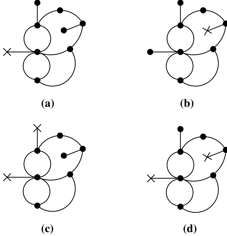
Figure 5. Samples of planar graphs with external legs (univalent vertices marked with a cross) and arbitrary valences, with respectively (a) one leg in the external face (b) one leg (anywhere) (c) two legs in the same (external) face (d) two-legs (one in the external face, the other anywhere).
