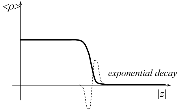
Figure 3. The mean density profile for models with quasiharmonic potential in the large N limit. The correction to the pure step function is shown by the dotted line. The effect of the correction is to form a double layer of charges near the edge.
