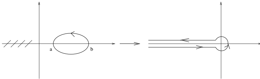
Figure 8. This shows the deformation of the contour needed to compute the planar resolvent of the Chern-Simons matrix integral. We pick a residue at z = p , and we have to encircle the singularity at the origin as well as the branch cut of the logarithm, which on the left hand side is represented by the dashed lines.
