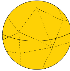
Figure 4. Triangulation of a two-dimensional sphere.
