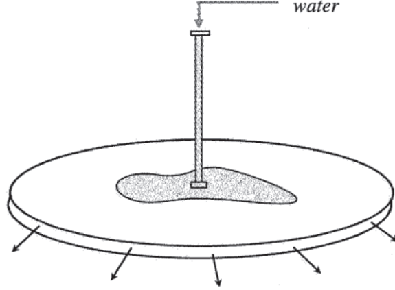
Figure 6. The Hele-Shaw cell.
