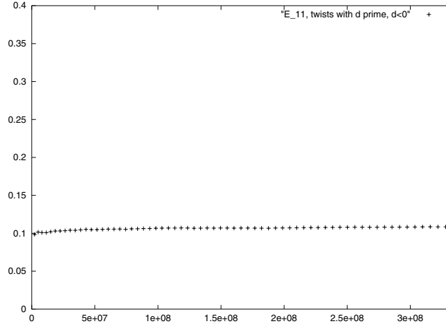
Figure 5. The l.h.s. of (87) divided by D^{3/4}(\log D)^{-5/8} . The calculations include only twists with d < 0 , d prime, and cases with even functional equation. While the picture is reasonably flat, \log(D) is almost constant for most of the interval in question. The flatness observed therefore reflects the main dependence on D^{3/4} . (From [12].)
