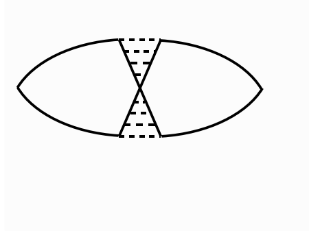
Figure 3. Cooperon: a singular correction to conductivity.
