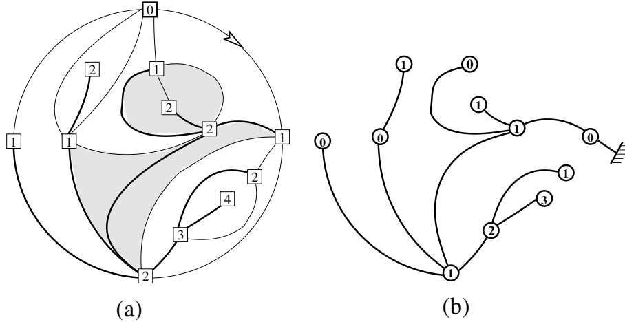
Figure 8. The bijection between planar quadrangulations and labeled trees. A planar rooted quadrangulation (a) and the natural labeling of its vertices by the geodesic distance to the origin vertex of the rooted edge (arrow). The confluent faces are shaded. The tree edges are represented in thick black lines, and connect all vertices with positive labels. Erasing all but these new edges and the vertices they connect leaves us with a labeled tree (b), which we root at the vertex corresponding to the end of the rooted edge of the initial quadrangulation. Finally, all labels of the tree are shifted by -1 .
