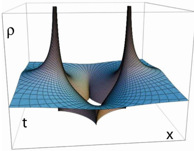
Figure 1. The density profile \rho(x, t) is shown for the EFP instanton. The density diverges at points (x, t) = (\pm R, 0) . The shape of the “Emptiness” is shown in Fig.2.
