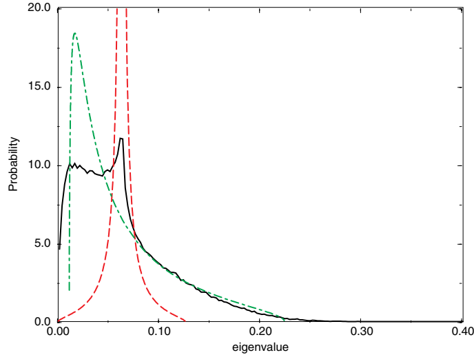
Figure 3. Density of eigenvalues of a Euclidean Random Matrix in three dimensions, density \rho = 0.1 . The function f is f(x) = (2\pi)^{-3/2} \exp(-x^2/2) , and the matrix is defined from eq.(48) with u = 0 . The full line is the result of a numerical simulation with N = 800 points, averaged over 200 samples. The dashed line is the result from a low density expansion introduced in [2]. The dash-dotted line is the result from the Gaussian variational approximation (RPA) to the field theory.
