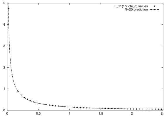
Figure 4. The value distribution of L_{E_{11}, d}(1) , for prime |d| , -788299808 < d < 0 , even functional equation, compared to equation (70), with N = 20 . Note the square-root divergence as w \rightarrow 0 . The L -function values have been normalized so that they have the same means as the random matrix value distributions. (From [12].)
