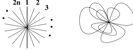
Figure 1. A star-diagram with one vertex and 2n out-coming half-edges stands for the integrand x^{2n} . In the second diagram, we have represented one non-zero contribution to \langle x^{2n} \rangle obtained by taking derivatives of \Sigma(s) by pairs represented as the corresponding pairings of half-edges into edges.
