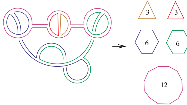
Figure 8. Unravelling a 3-valent graph.
