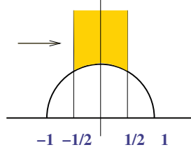
Figure 3. Moduli space of a torus, \mathcal{M}_{1,0} .
