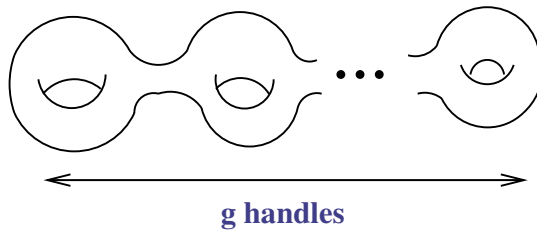
Figure 1. A generic compact Riemann surface.
