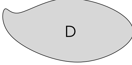
Figure 2. The support of eigenvalues.
