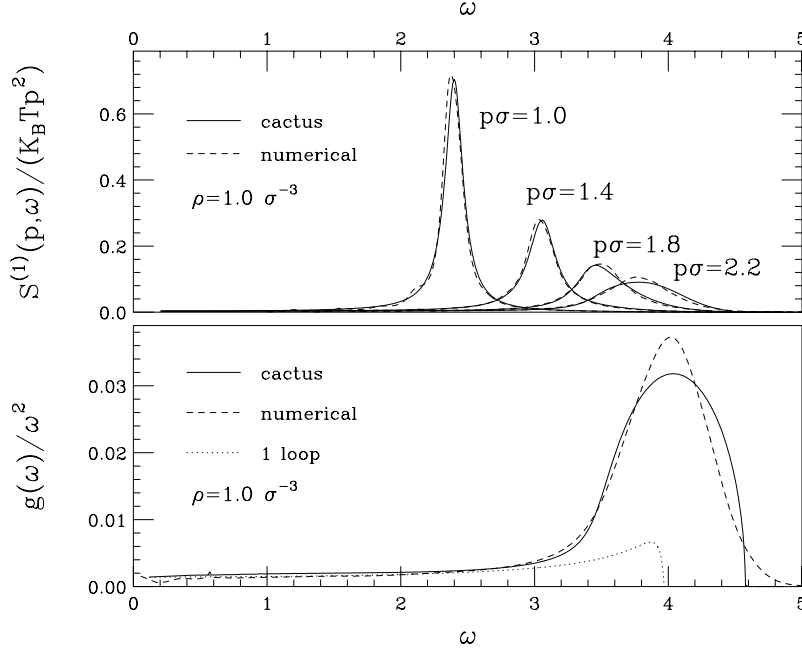
Figure 5. Top: dynamic structure factor as obtained from Eq.(121) (full line) and from simulations [7] (dashes). Bottom: the density of states divided by \omega^2 (Debye behavior) as obtained from Eq.(123) (full line), simulations (dashes), and first order in the 1/\rho expansion (dots).
