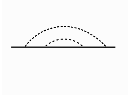
Figure 2. Typical diagrams for the Green function in a disordered metal.
