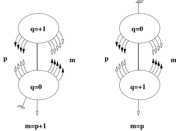
Figure 7. The only two possibilities for the environment of an edge in a 4-valent blossom-tree, obtained by cutting a two-leg planar 4-valent graph. The edge separates the tree into a top and a bottom piece. The first leg of the graph is chosen to be in the bottom piece. The two cases correspond to whether the cutting process stops in the top (a) or bottom (b) piece. We have represented in both cases only the leaves unmatched within each piece. In each case, the position of the root (second leg) is fixed by the fact that any 4-valent tree must have an even number of leaves (including the root). We have indicated the corresponding charges q = 0 or +1 of the top and bottom pieces.
