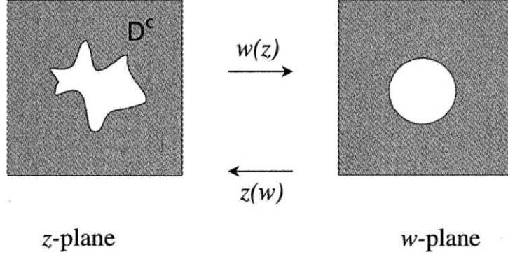
Figure 5. The mutually inverse conformal maps w(z) and z(w) .
